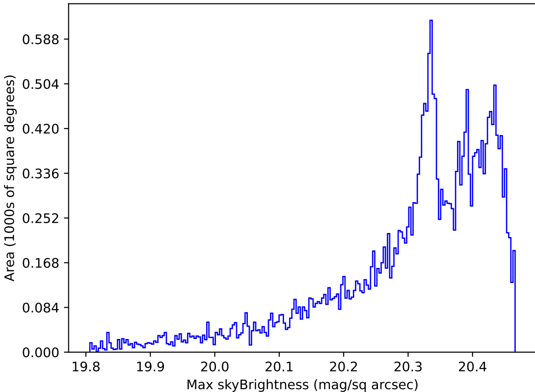
too_10_4v3.4_10yrs All sky i band: Max skyBrightness
