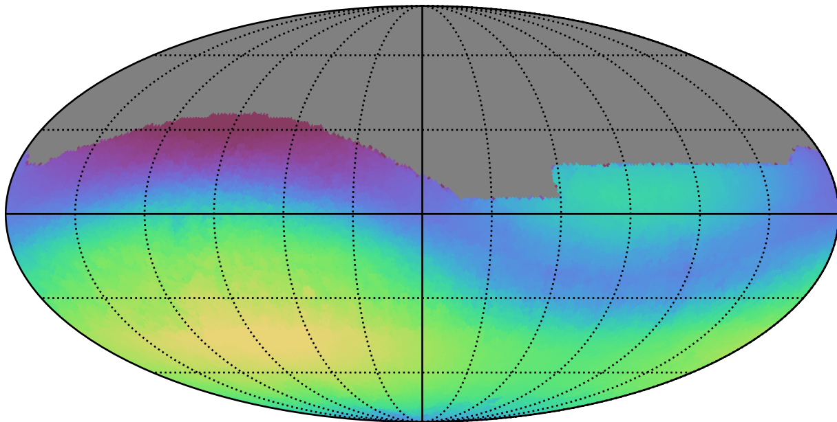
too_10_4v3.4_10yrs All sky g band: Max skyBrightness
