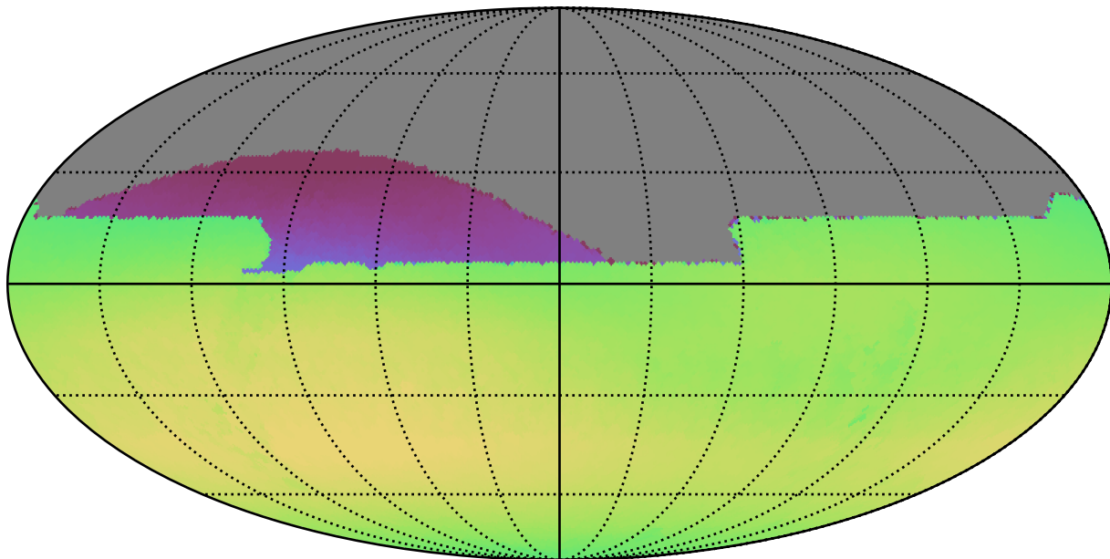
too_10_4v3.4_10yrs All sky all bands: Max skyBrightness
