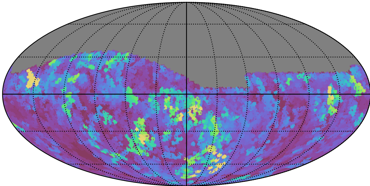
too_10_4v3.4_10yrs Yr 1 z band: Max seeingGeom
