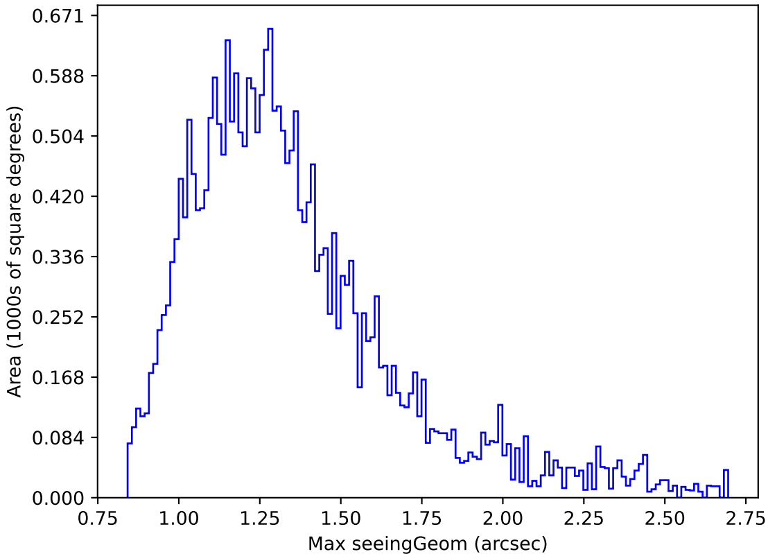
too_10_4v3.4_10yrs Yr 1 z band: Max seeingGeom
