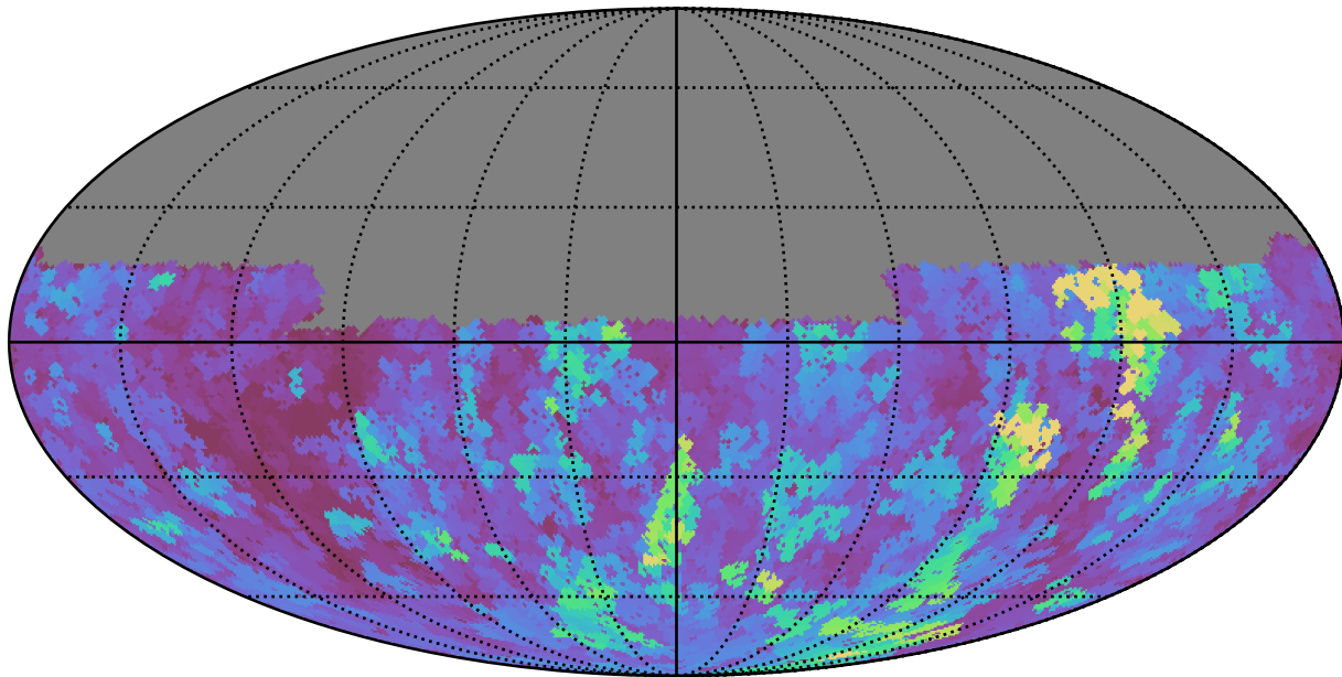
too_10_4v3.4_10yrs Yr 1 u band: Max seeingGeom
