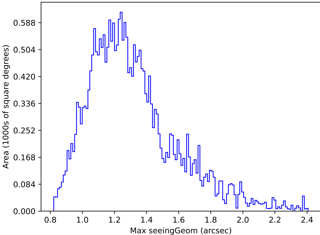
too_10_4v3.4_10yrs Yr 1 g band: Max seeingGeom
