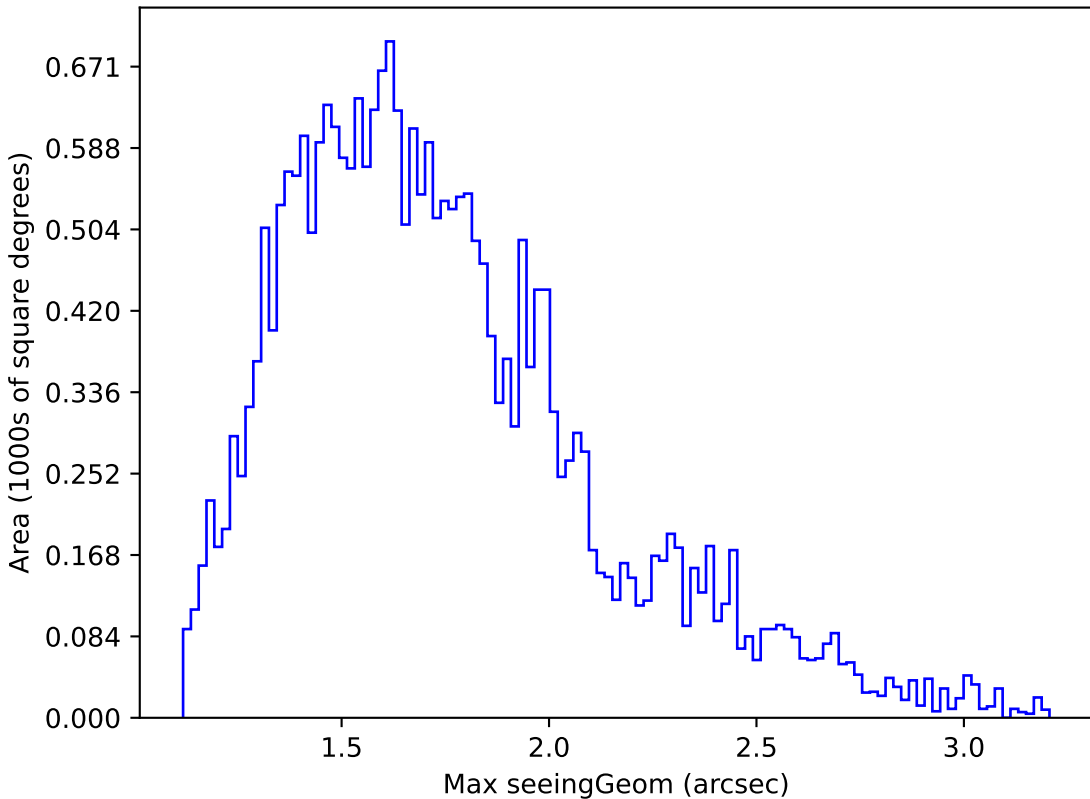
too_10_4v3.4_10yrs Yr 1 all bands: Max seeingGeom
