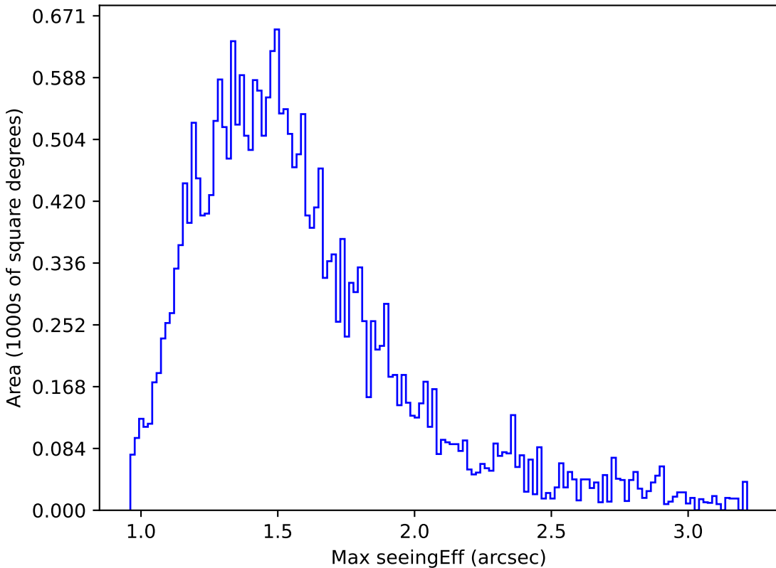
too_10_4v3.4_10yrs Yr 1 z band: Max seeingEff
