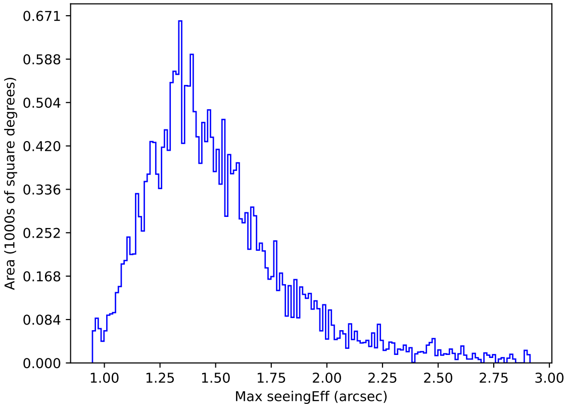
too_10_4v3.4_10yrs Yr 1 y band: Max seeingEff
