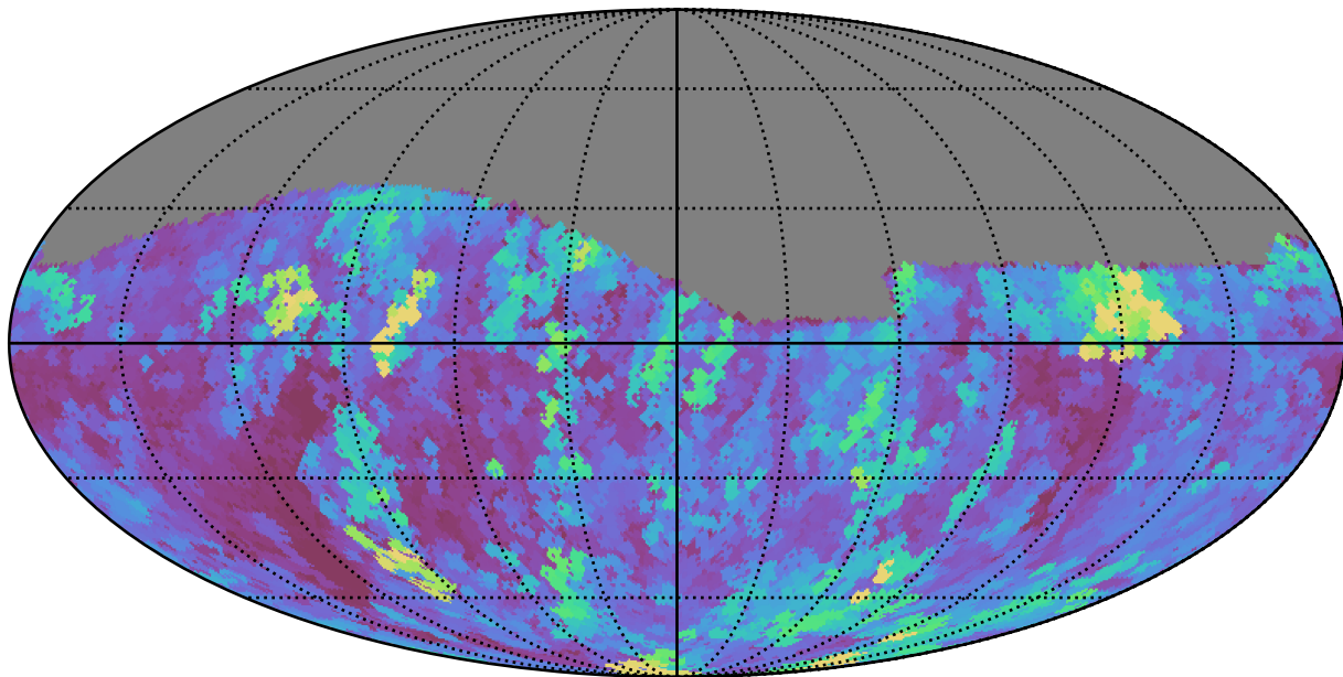
too_10_4v3.4_10yrs Yr 1 r band: Max seeingEff
