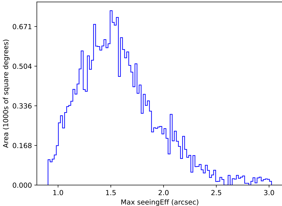
too_10_4v3.4_10yrs Yr 1 r band: Max seeingEff
