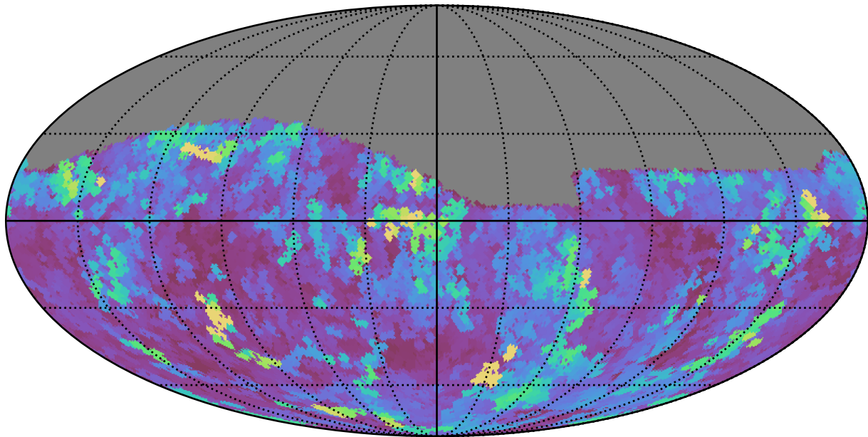
too_10_4v3.4_10yrs Yr 1 i band: Max seeingEff
