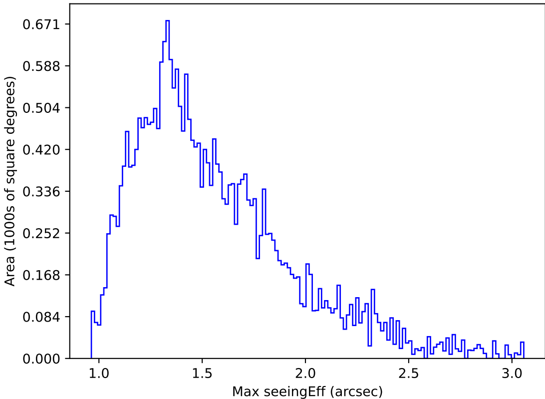
too_10_4v3.4_10yrs Yr 1 i band: Max seeingEff
