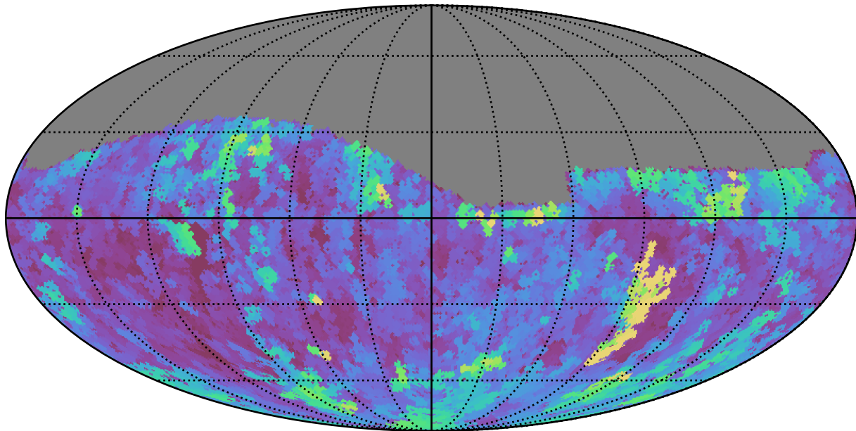
too_10_4v3.4_10yrs Yr 1 g band: Max seeingEff
