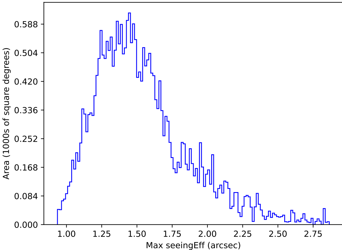
too_10_4v3.4_10yrs Yr 1 g band: Max seeingEff
