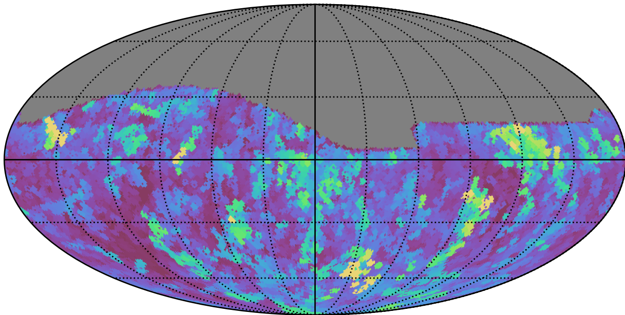
too_10_4v3.4_10yrs Yr 1 all bands: Max seeingEff
