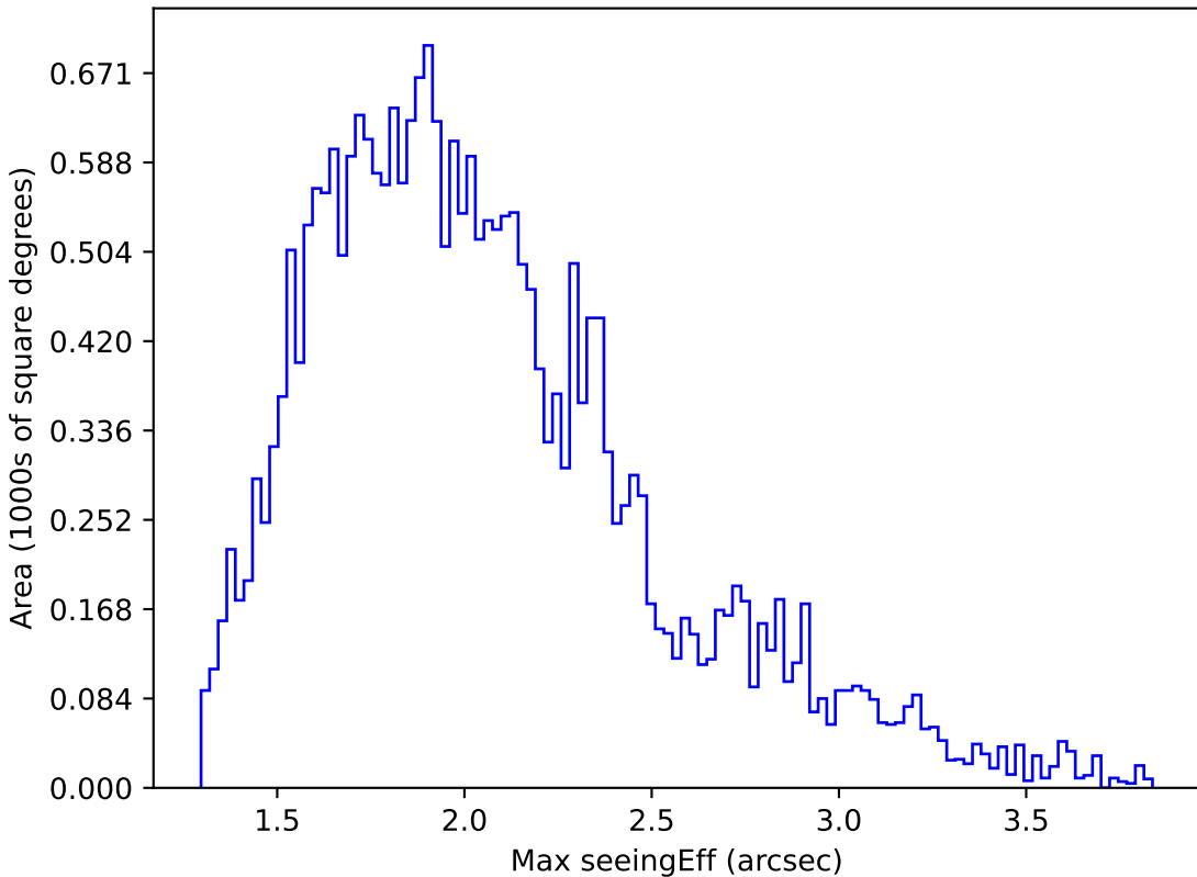
too_10_4v3.4_10yrs Yr 1 all bands: Max seeingEff
