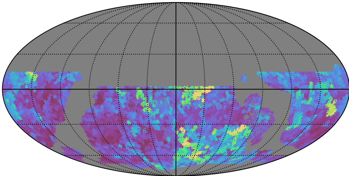
too_10_4v3.4_10yrs WFD z band: Max seeingEff
