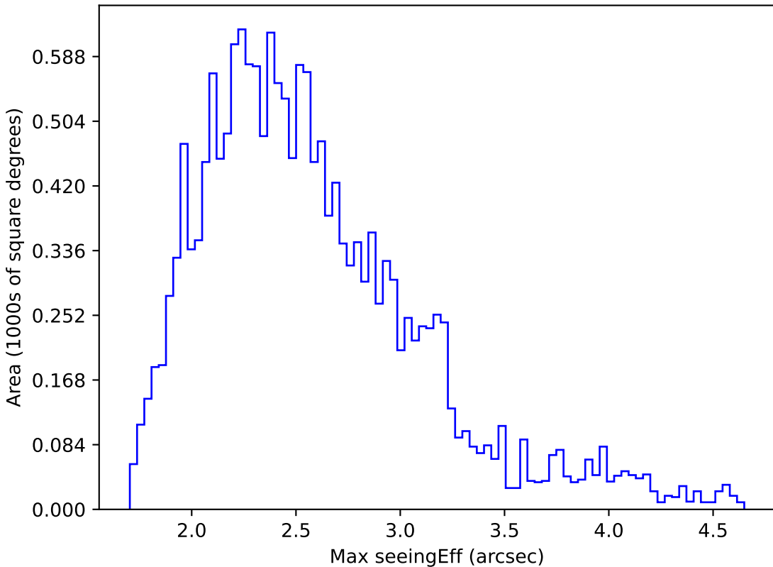
too_10_4v3.4_10yrs WFD z band: Max seeingEff
