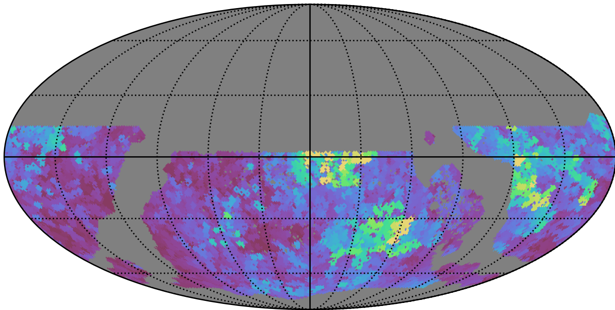
too_10_4v3.4_10yrs WFD y band: Max seeingEff
