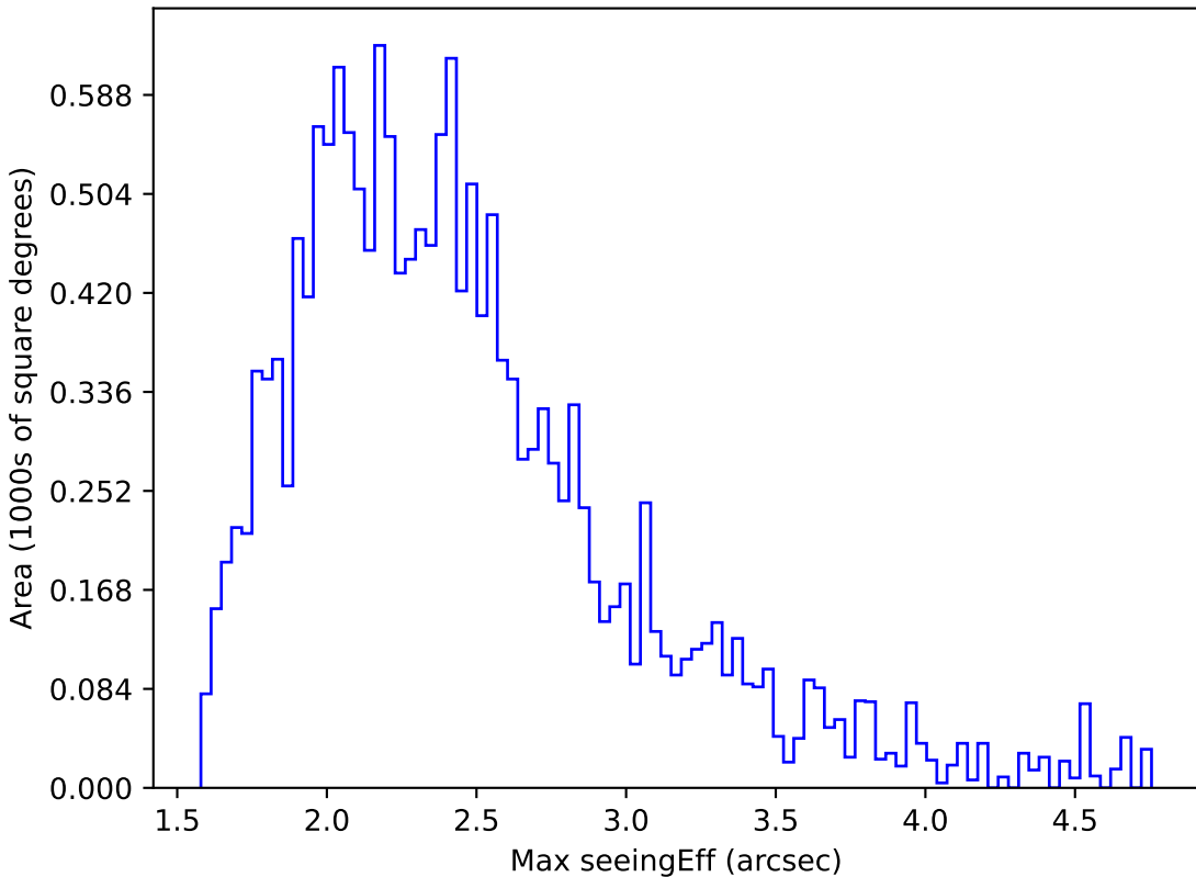
too_10_4v3.4_10yrs WFD y band: Max seeingEff
