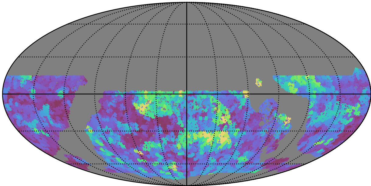
too_10_4v3.4_10yrs WFD u band: Max seeingEff
