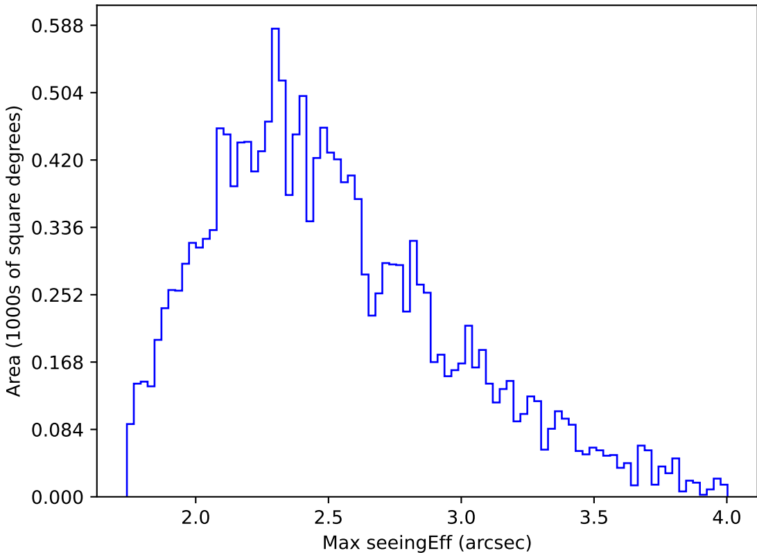
too_10_4v3.4_10yrs WFD u band: Max seeingEff
