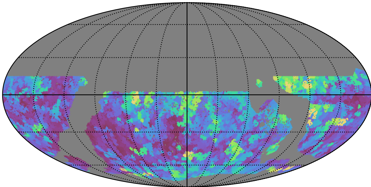
too_10_4v3.4_10yrs WFD r band: Max seeingEff
