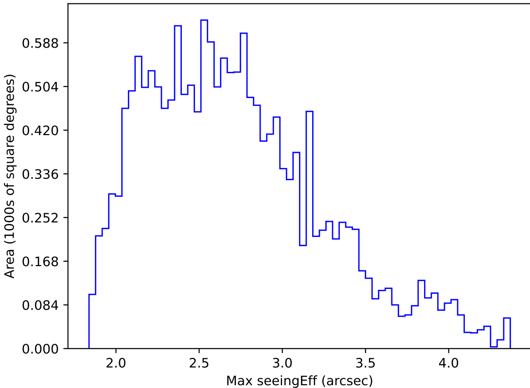
too_10_4v3.4_10yrs WFD r band: Max seeingEff
