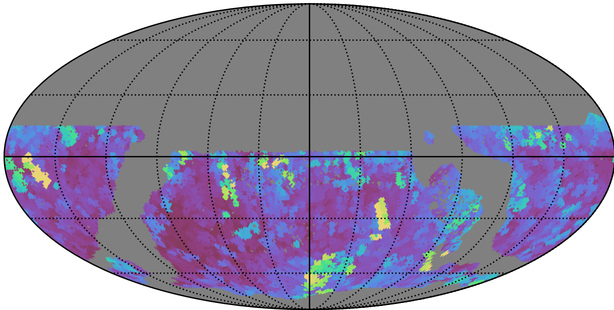
too_10_4v3.4_10yrs WFD i band: Max seeingEff
