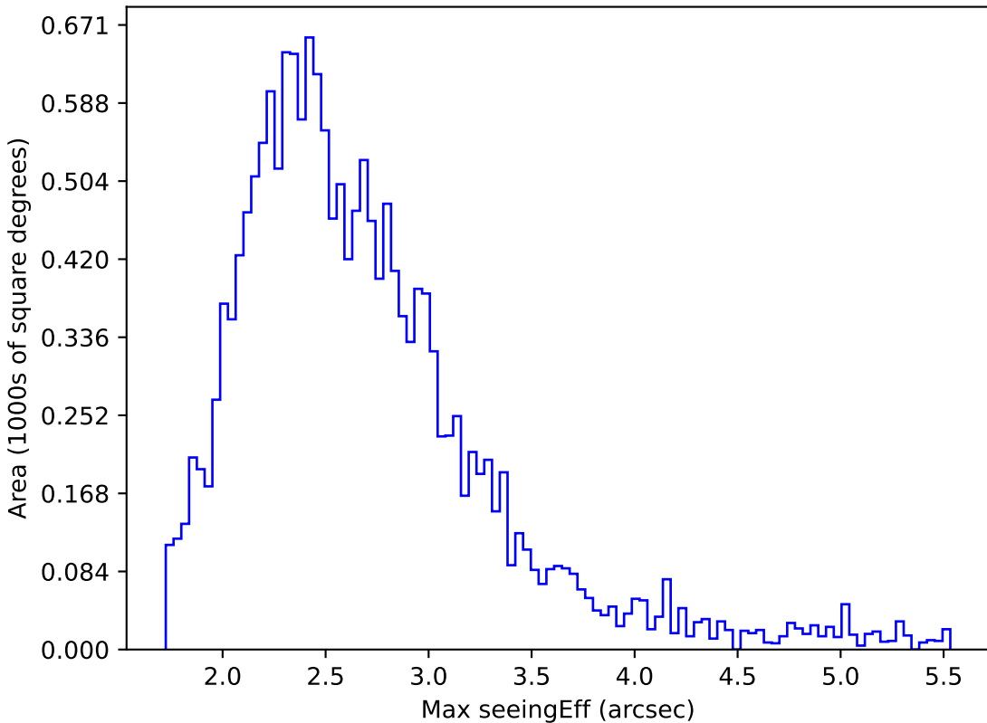
too_10_4v3.4_10yrs WFD i band: Max seeingEff
