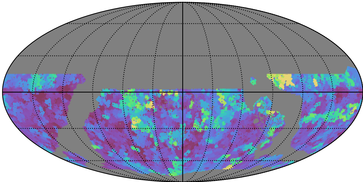
too_10_4v3.4_10yrs WFD g band: Max seeingEff
