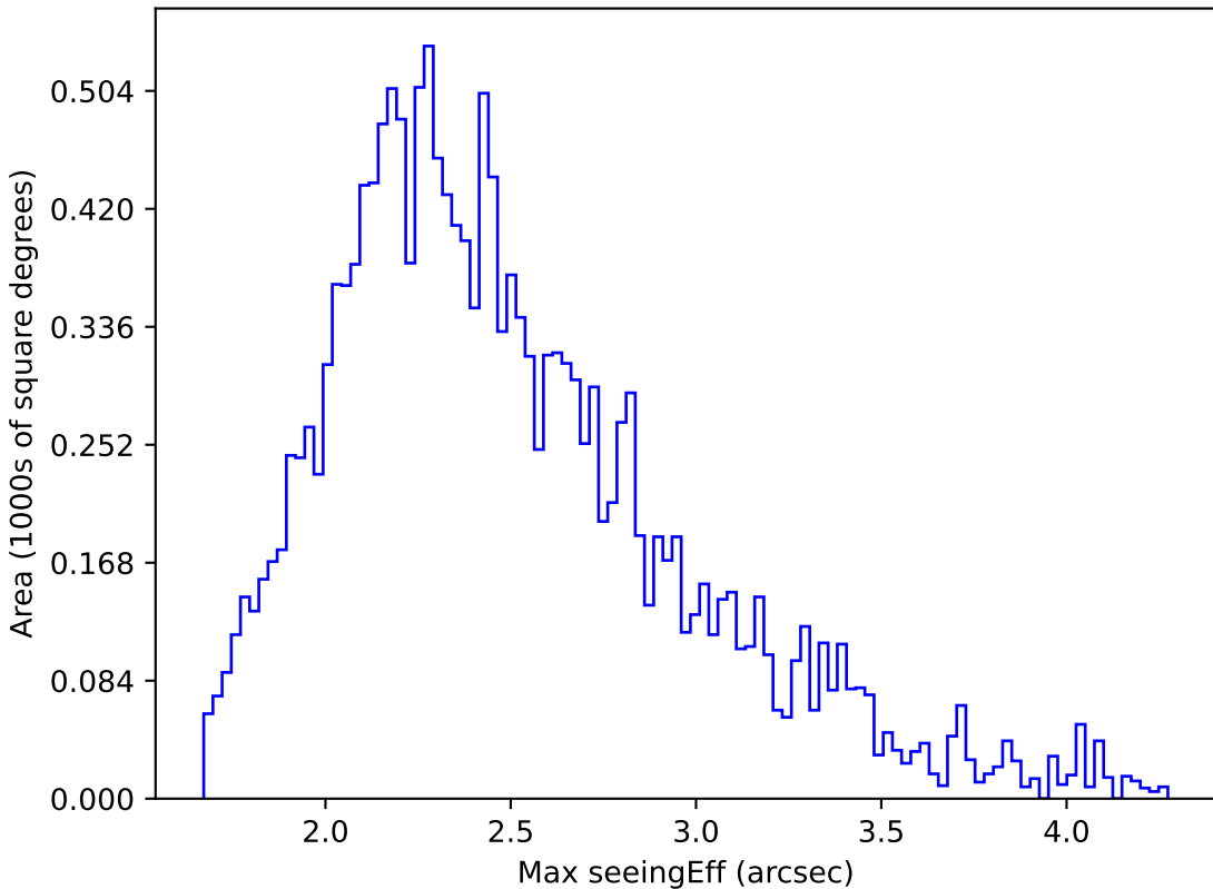
too_10_4v3.4_10yrs WFD g band: Max seeingEff
