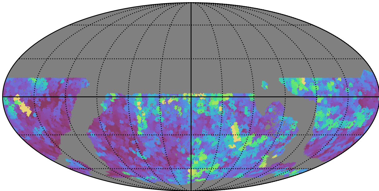
too_10_4v3.4_10yrs WFD all bands: Max seeingEff
