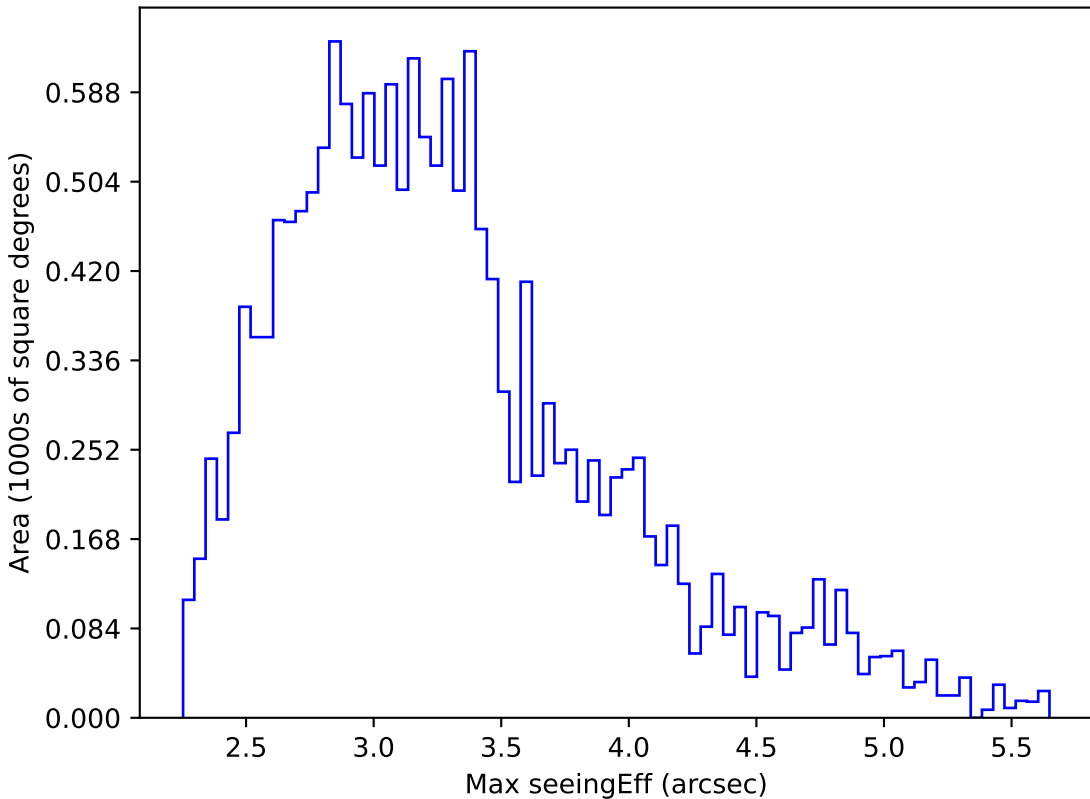
too_10_4v3.4_10yrs WFD all bands: Max seeingEff
