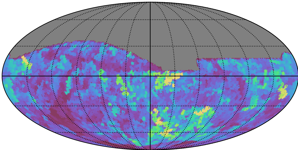
too_10_4v3.4_10yrs All sky z band: Max seeingEff
