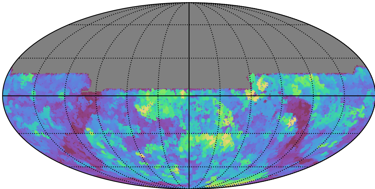
too_10_4v3.4_10yrs All sky u band: Max seeingEff
