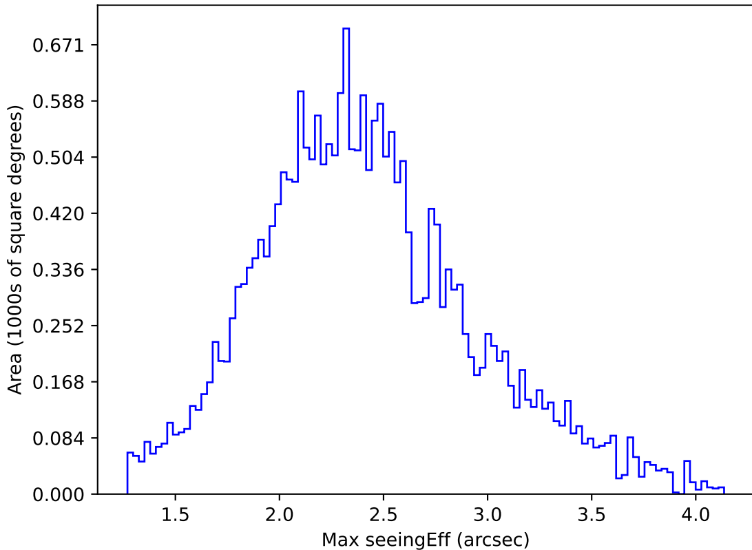
too_10_4v3.4_10yrs All sky u band: Max seeingEff
