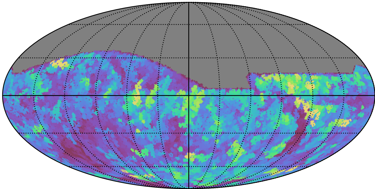
too_10_4v3.4_10yrs All sky r band: Max seeingEff
