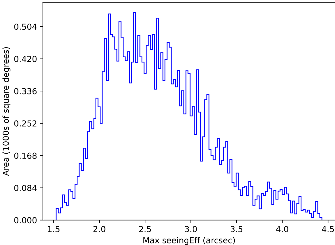
too_10_4v3.4_10yrs All sky r band: Max seeingEff
