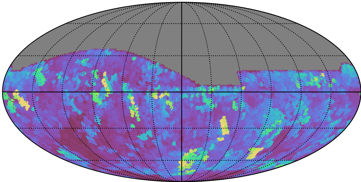
too_10_4v3.4_10yrs All sky i band: Max seeingEff
