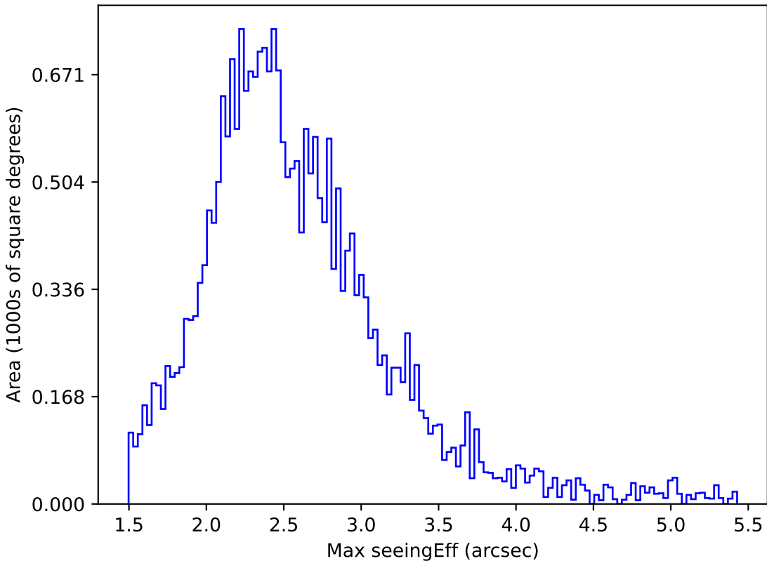
too_10_4v3.4_10yrs All sky i band: Max seeingEff
