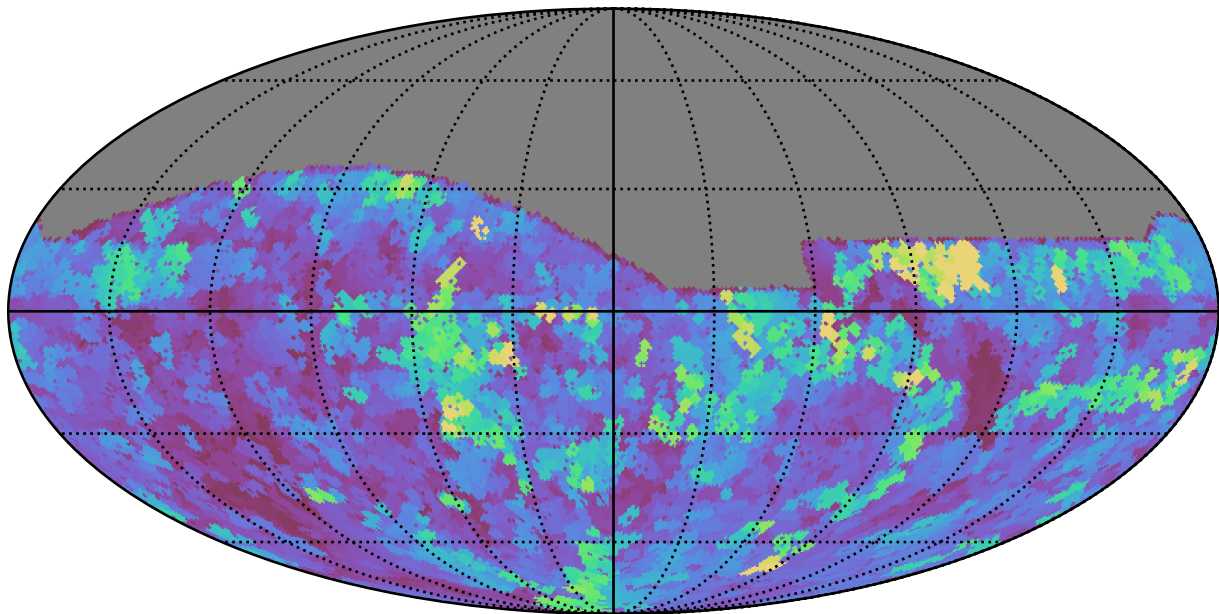
too_10_4v3.4_10yrs All sky g band: Max seeingEff
