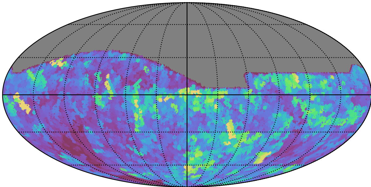
too_10_4v3.4_10yrs All sky all bands: Max seeingEff
