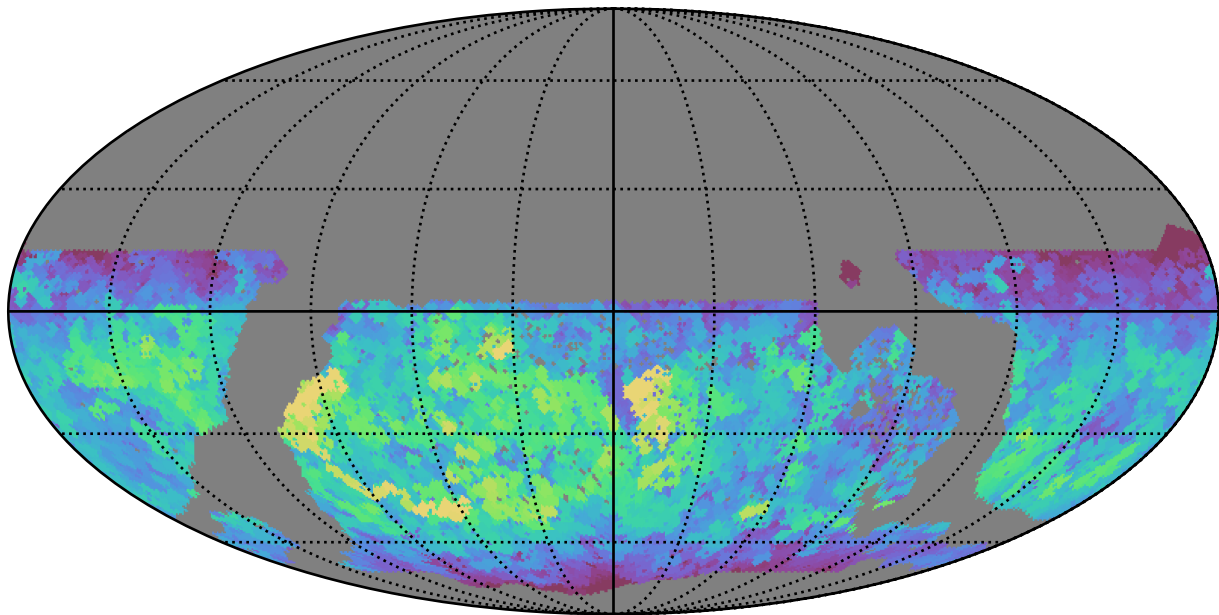
too_10_4v3.4_10yrs WFD y band: Max saturation_mag
