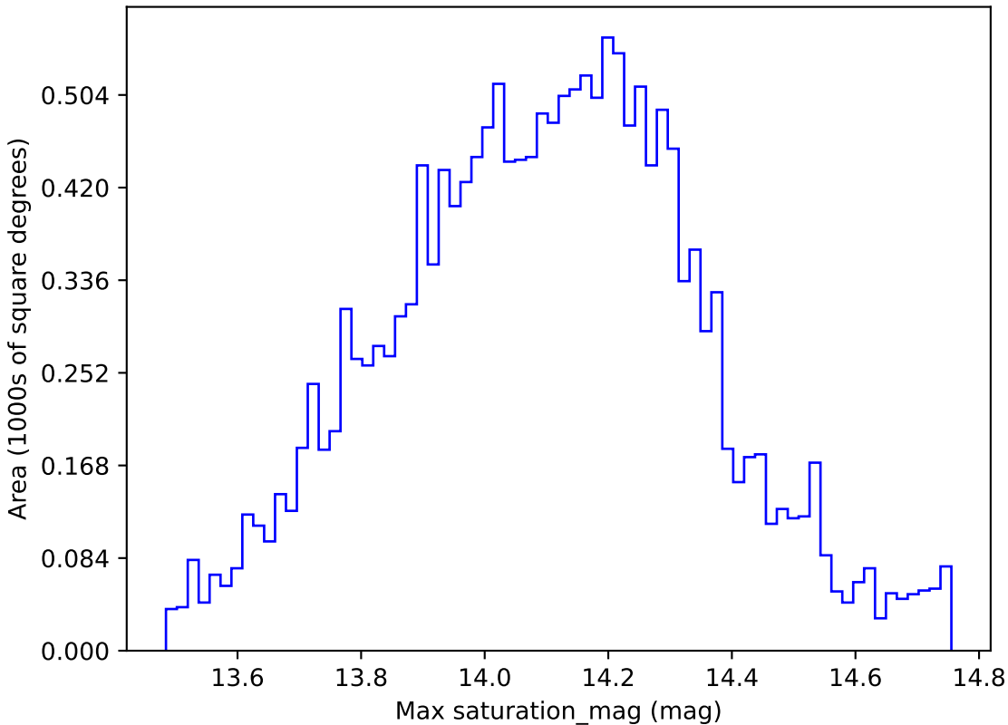
too_10_4v3.4_10yrs WFD u band: Max saturation_mag
