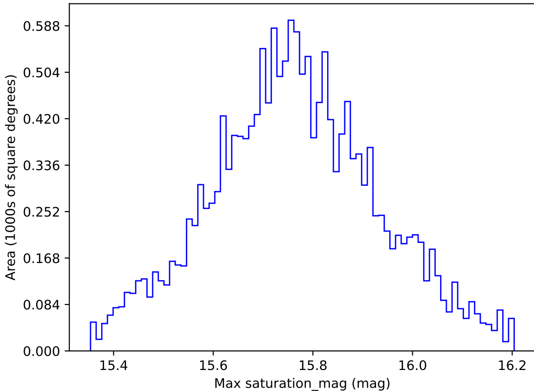
too_10_4v3.4_10yrs WFD r band: Max saturation_mag
