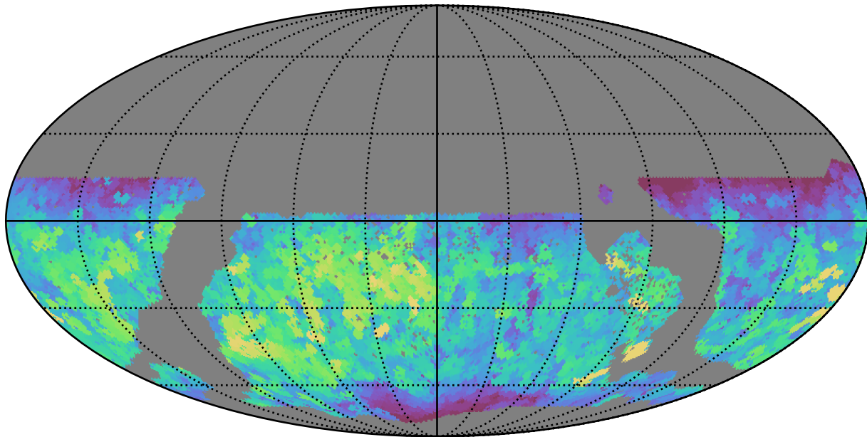
too_10_4v3.4_10yrs WFD i band: Max saturation_mag
