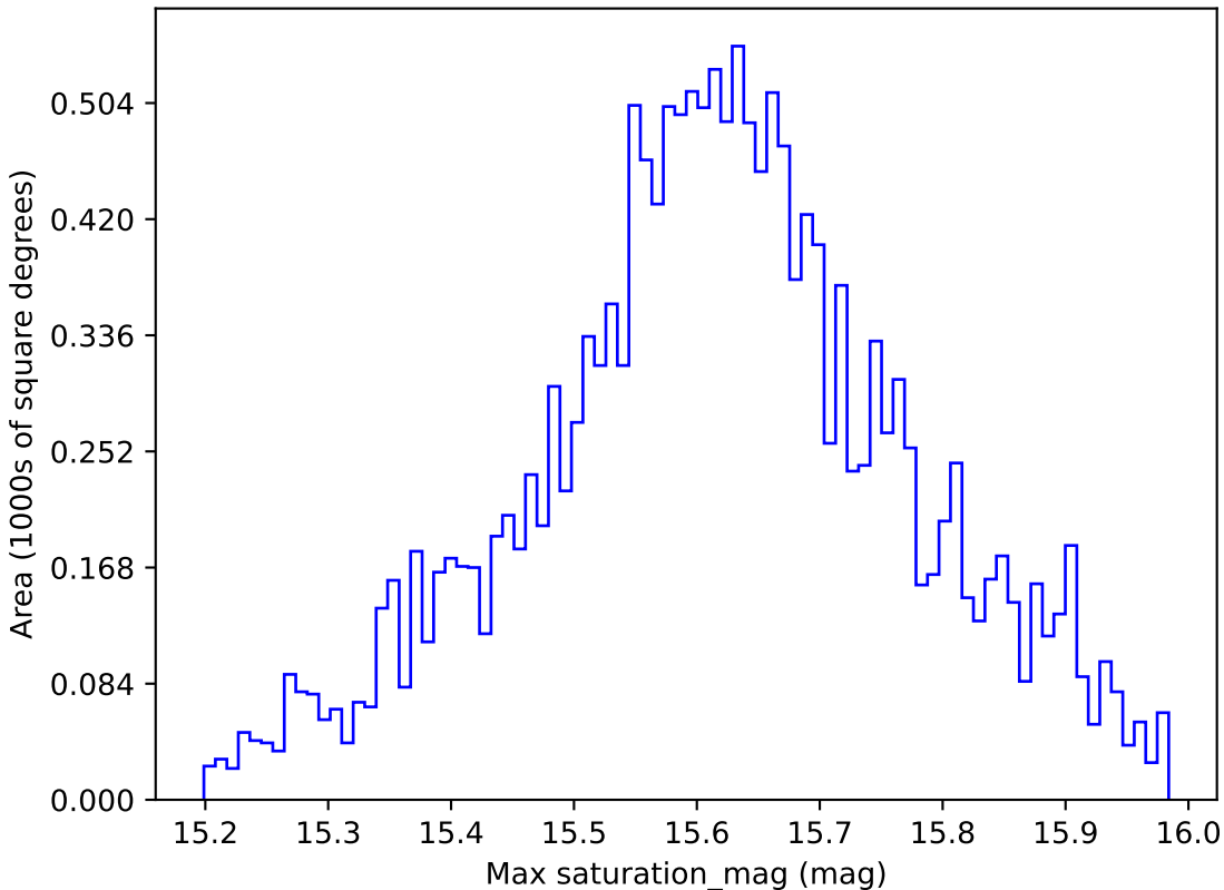
too_10_4v3.4_10yrs WFD i band: Max saturation_mag
