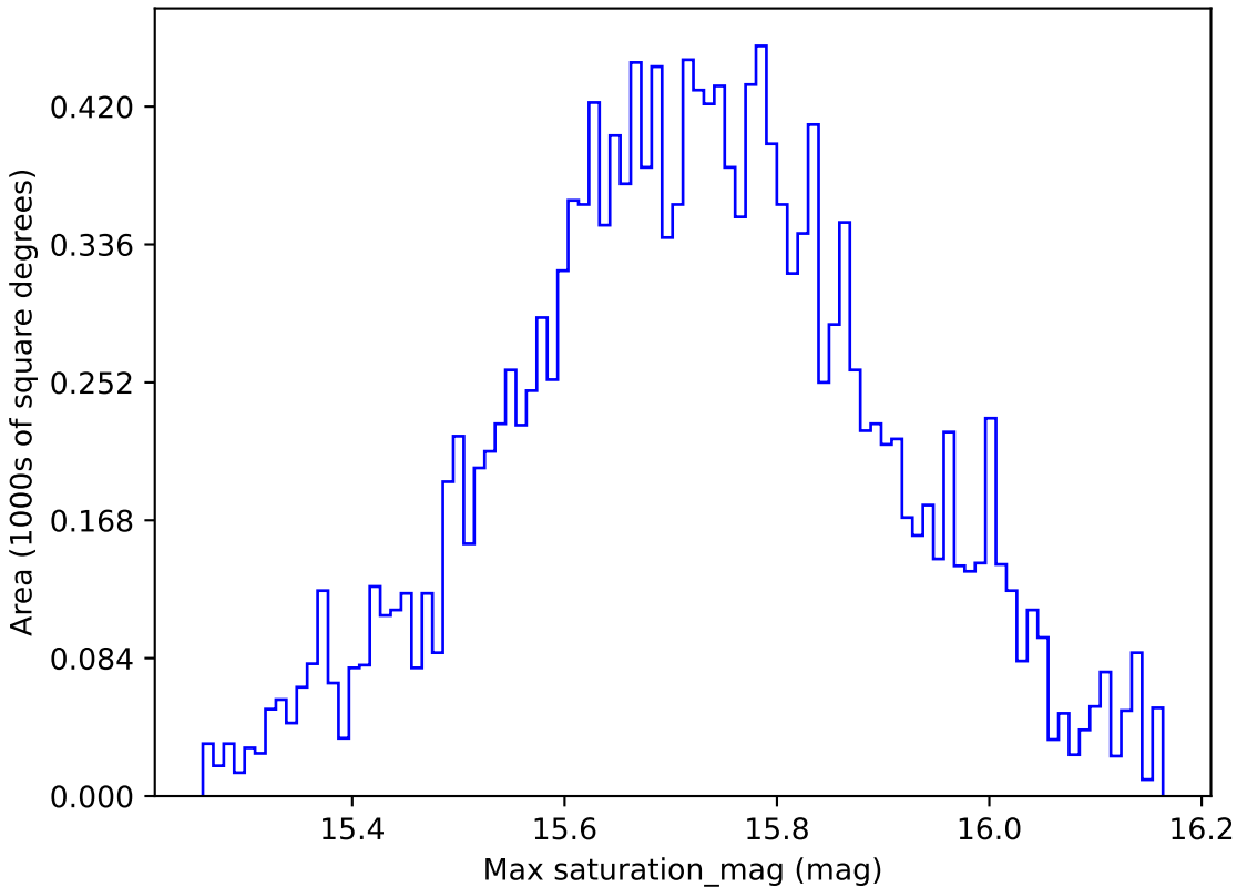
too_10_4v3.4_10yrs WFD g band: Max saturation_mag
