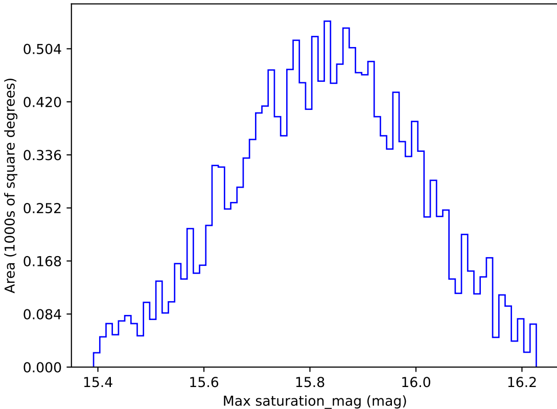
too_10_4v3.4_10yrs WFD all bands: Max saturation_mag
