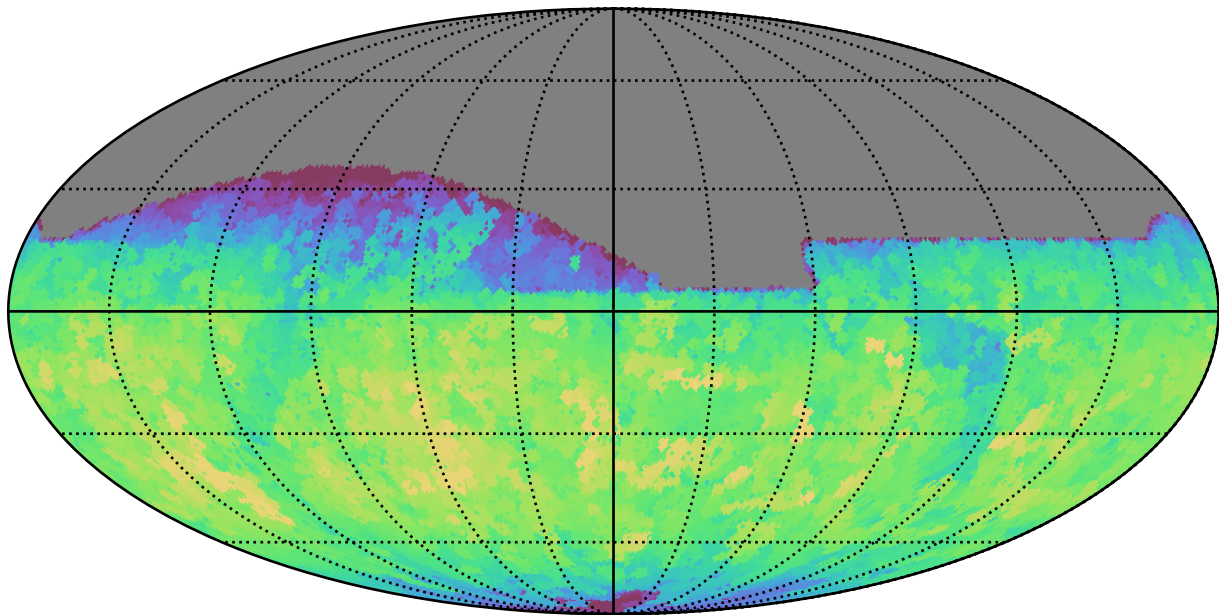
too_10_4v3.4_10yrs All sky z band: Max saturation_mag
