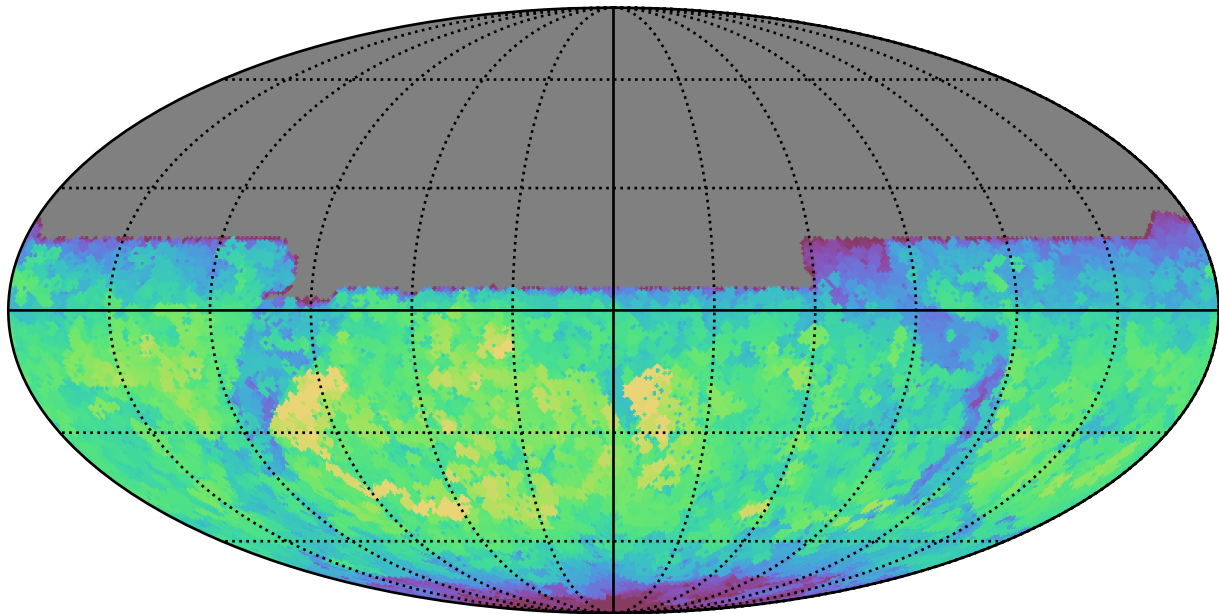
too_10_4v3.4_10yrs All sky y band: Max saturation_mag
